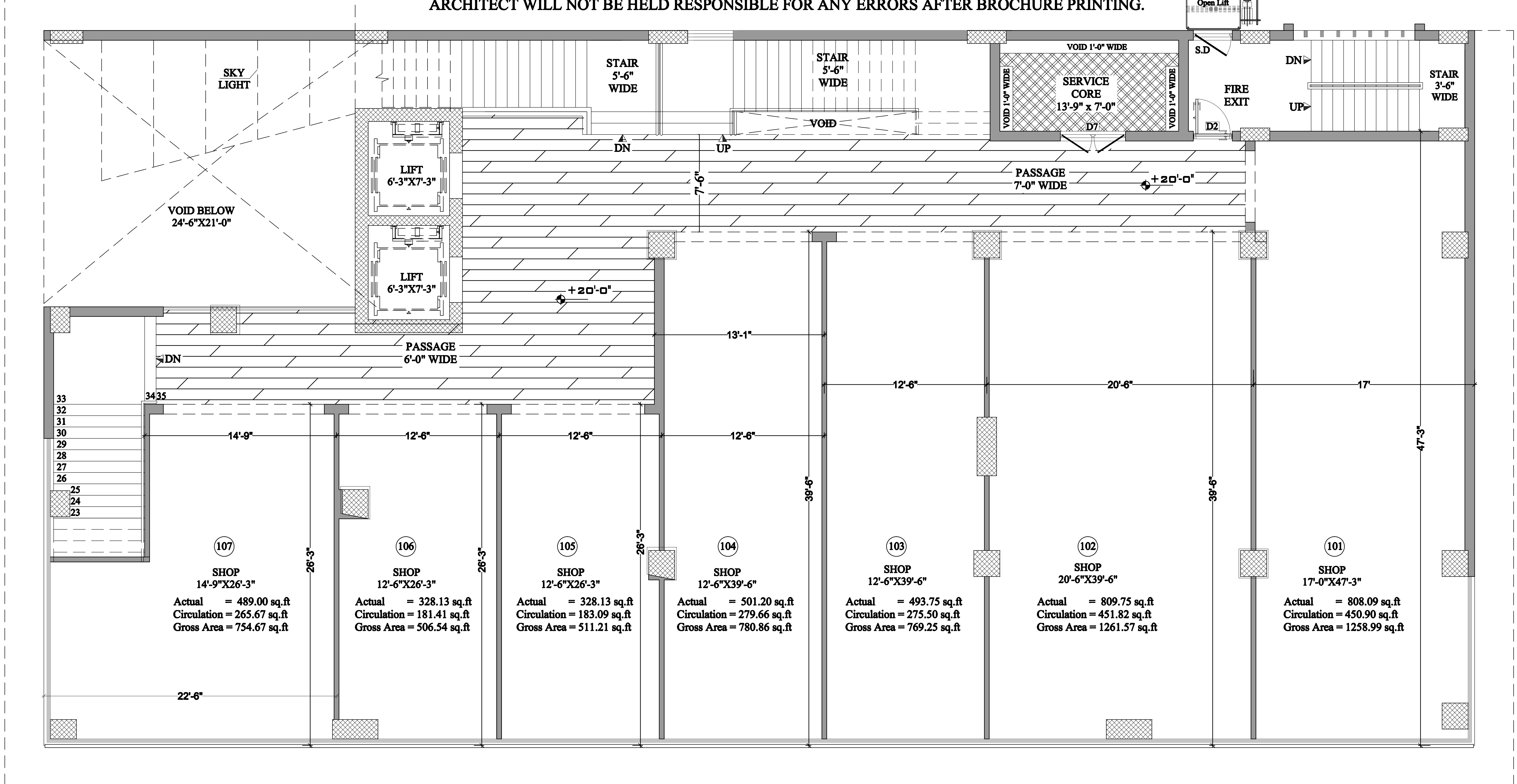
ALL DIMENSIONS INCLUDING WALLS
