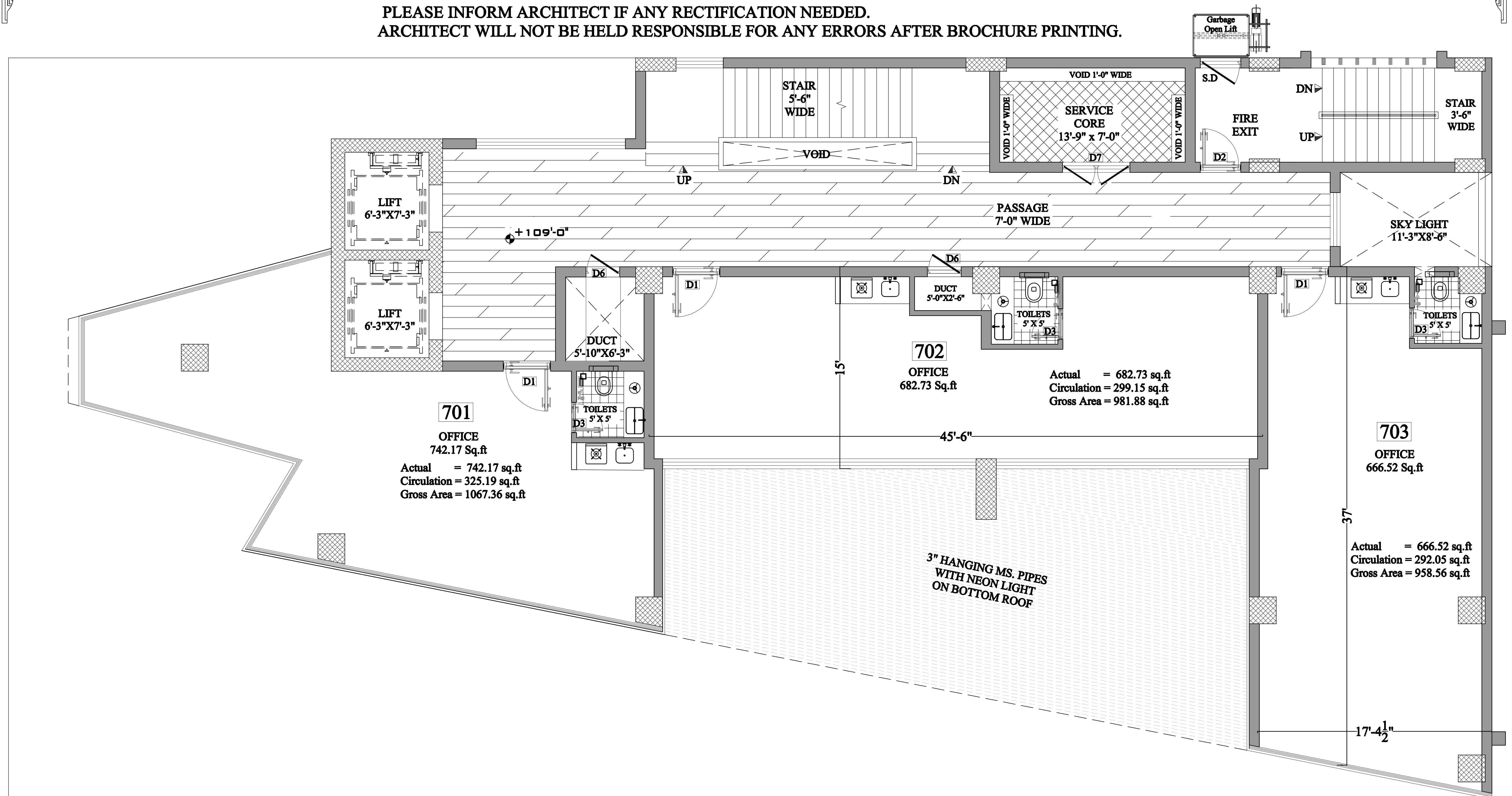
7th FLOOR PLAN ALL DIMENSIONS INCLUDING WALLS
