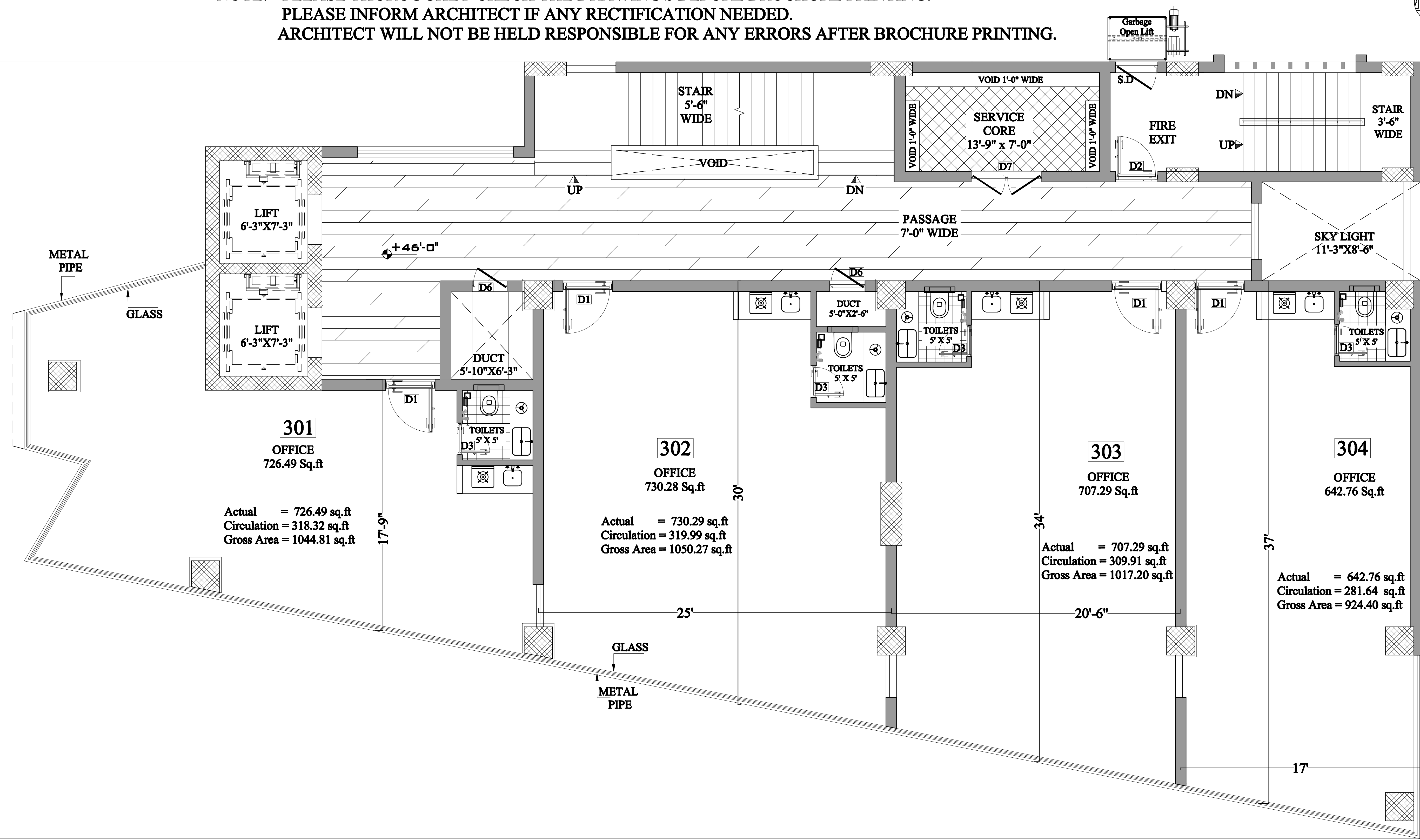
3rd FLOOR PLAN ALL DIMENSIONS INCLUDING WALLS
