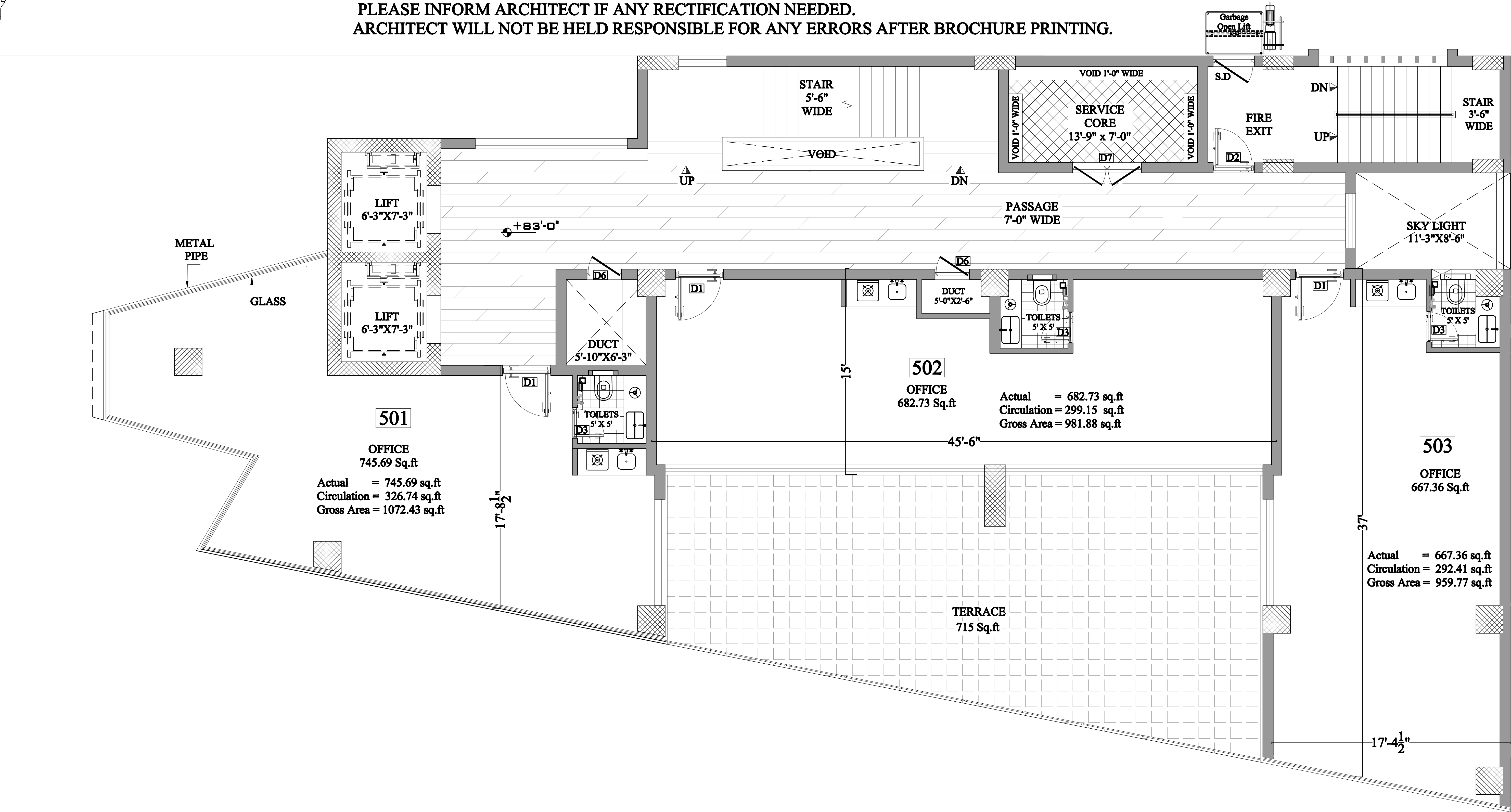
5th FLOOR PLAN ALL DIMENSIONS INCLUDING WALLS
