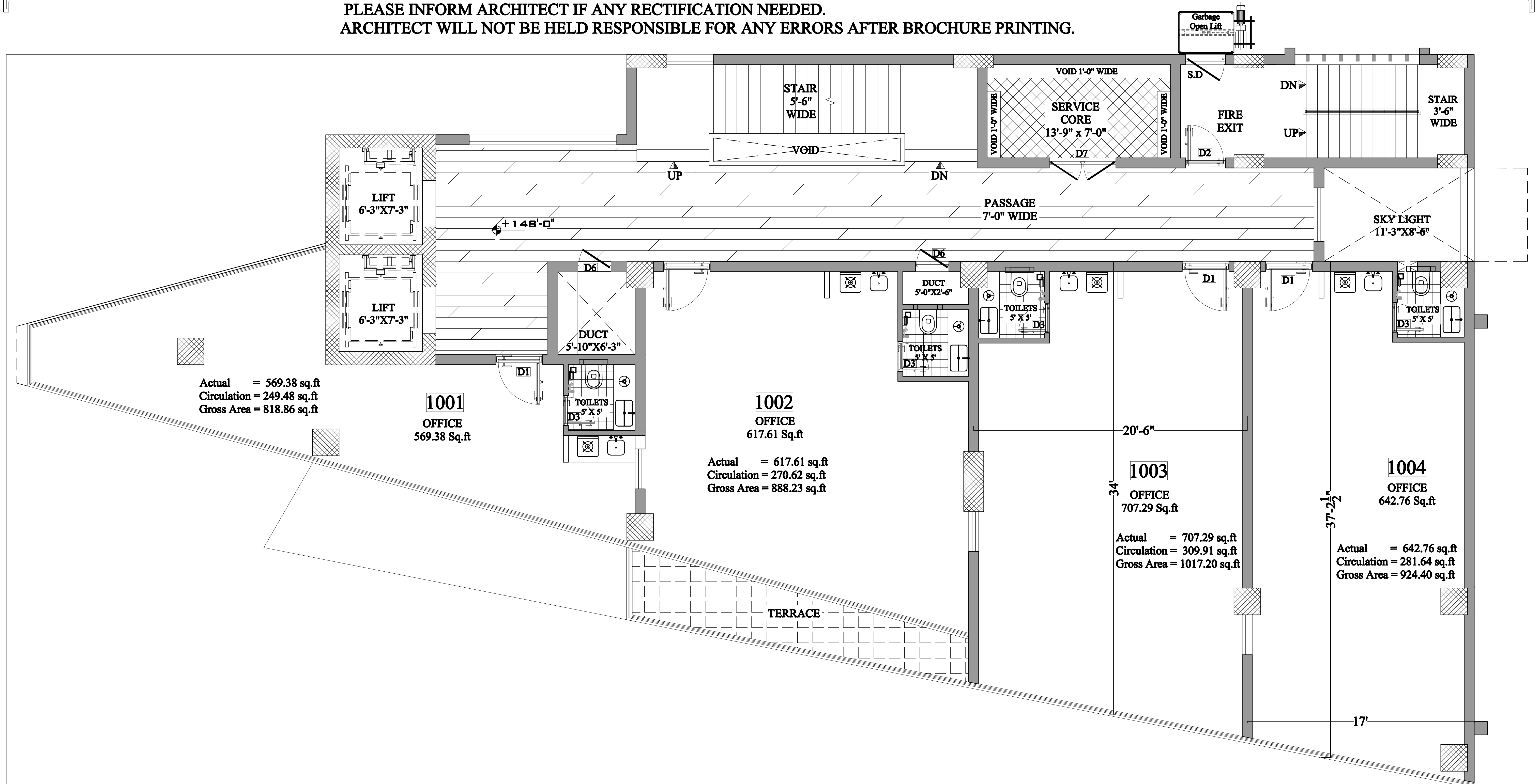
10th FLOOR PLAN ALL DIMENSIONS INCLUDING WALLS
