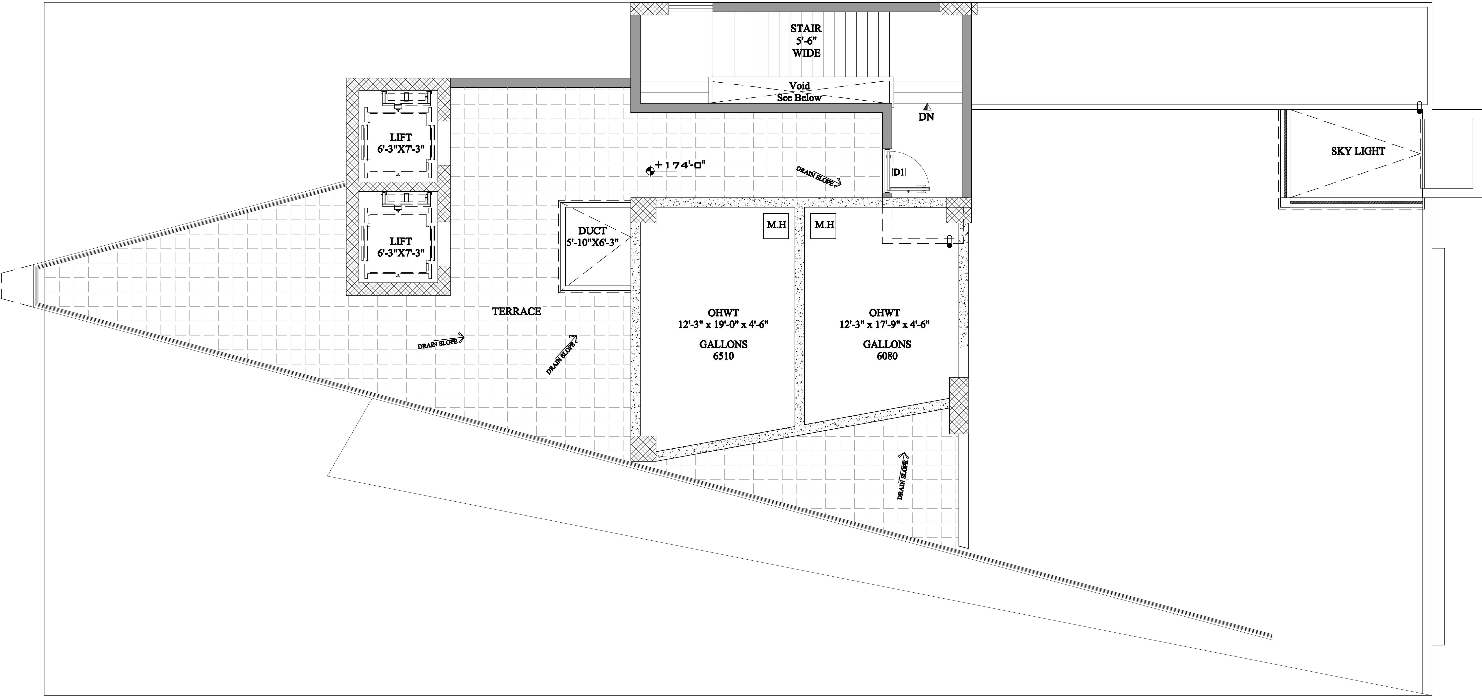
MUMTY FLOOR PLAN ALL DIMENSIONS INCLUDING WALLS
