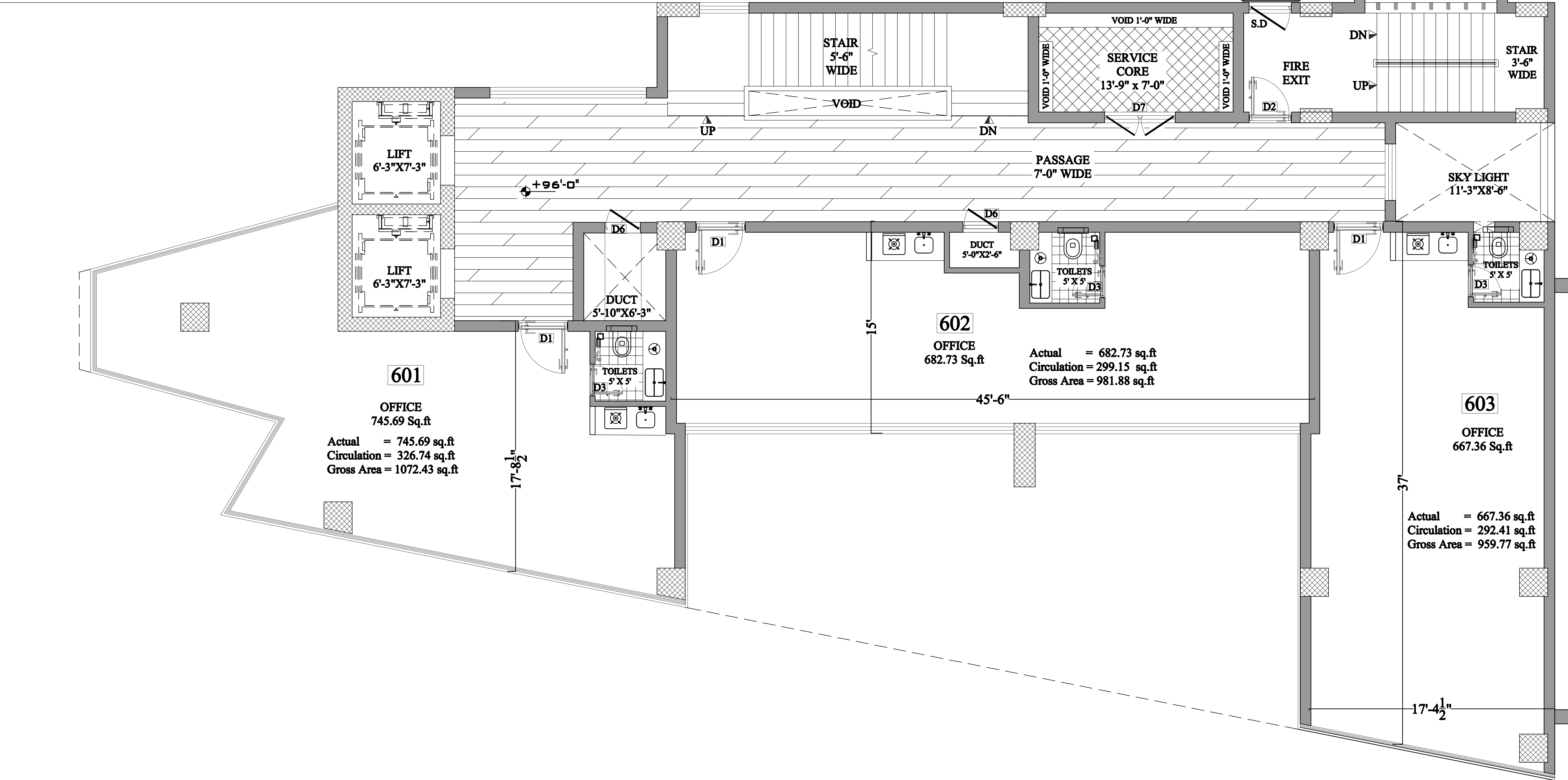
6th FLOOR PLAN ALL DIMENSIONS INCLUDING WALLS
