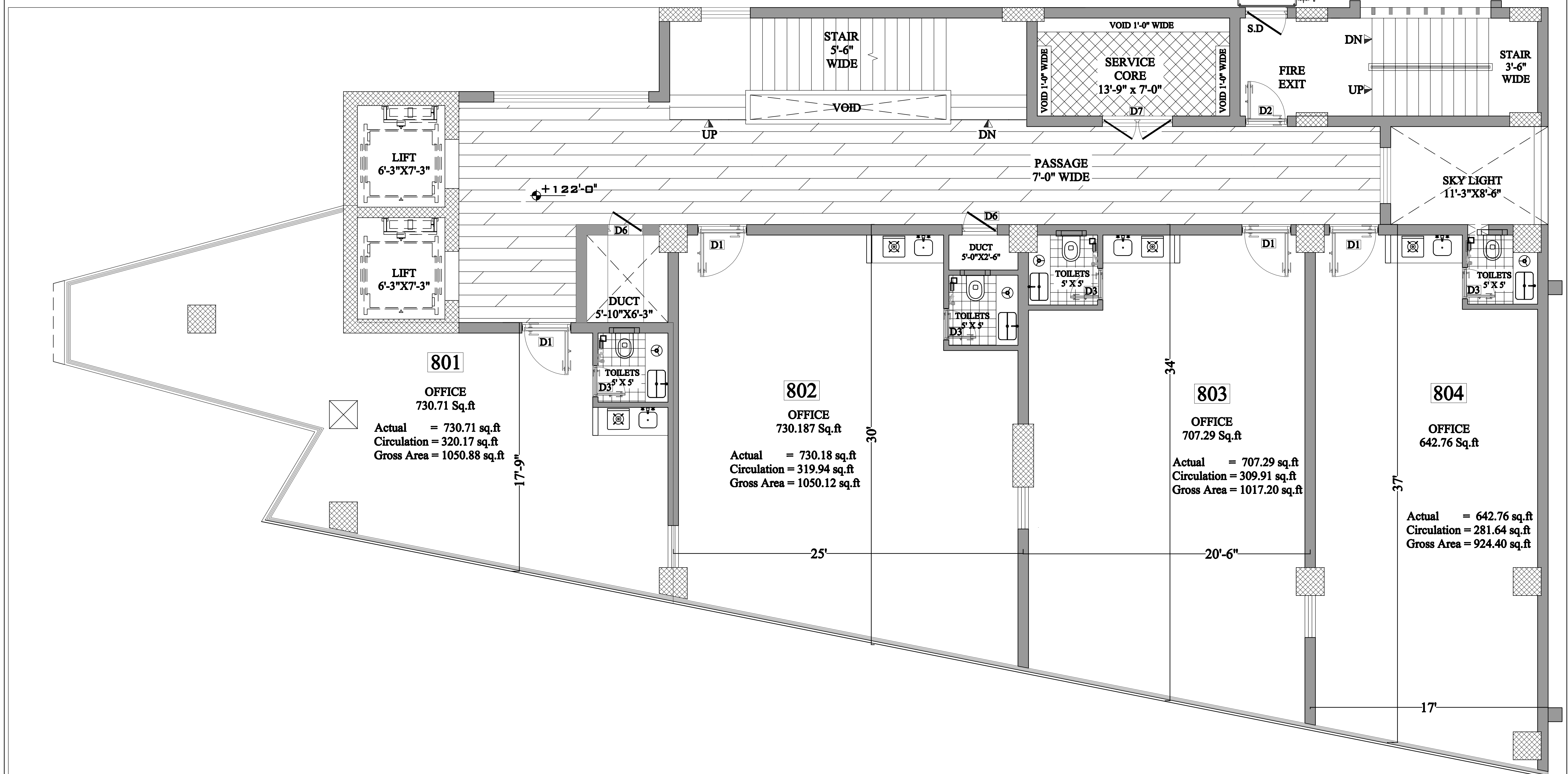
ALL DIMENSIONS INCLUDING WALLS
